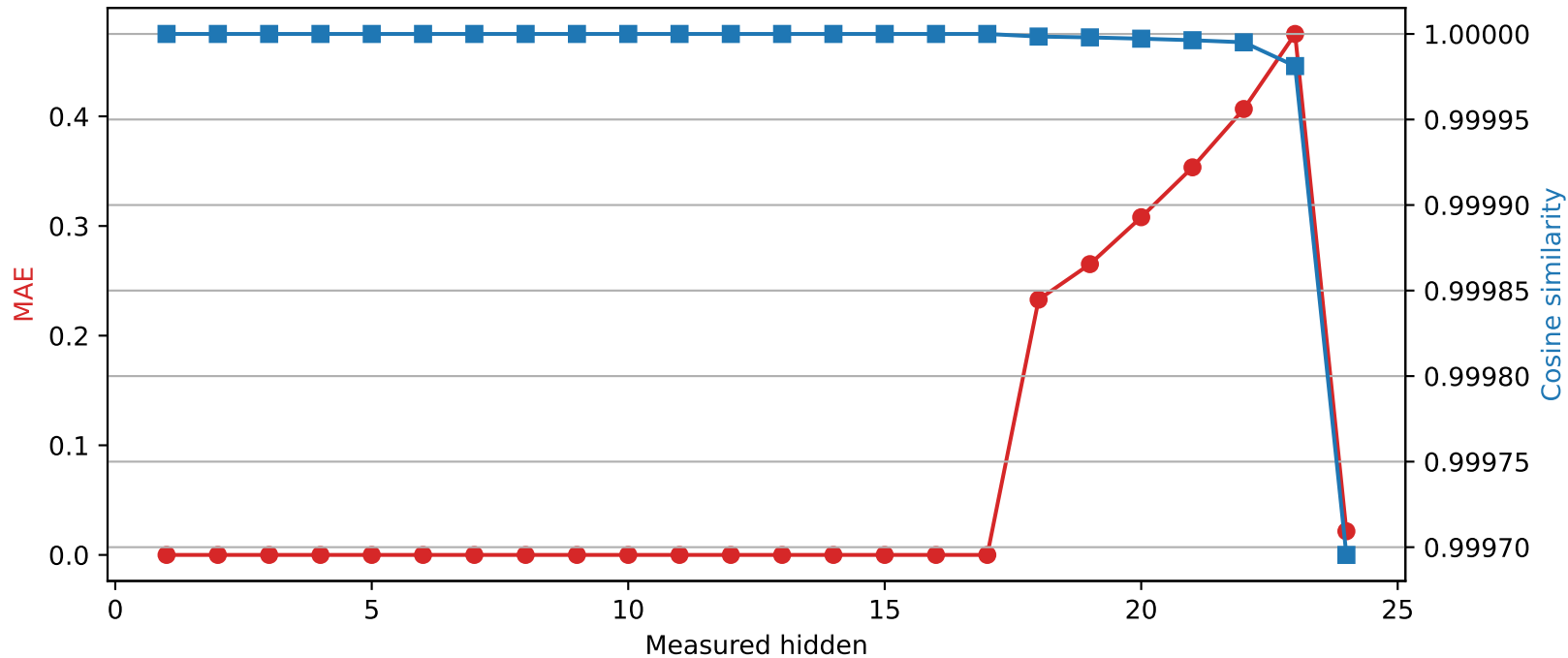
SmolLM2-1.7B-Instruct | Quantized layer 17 | float32 → int8
