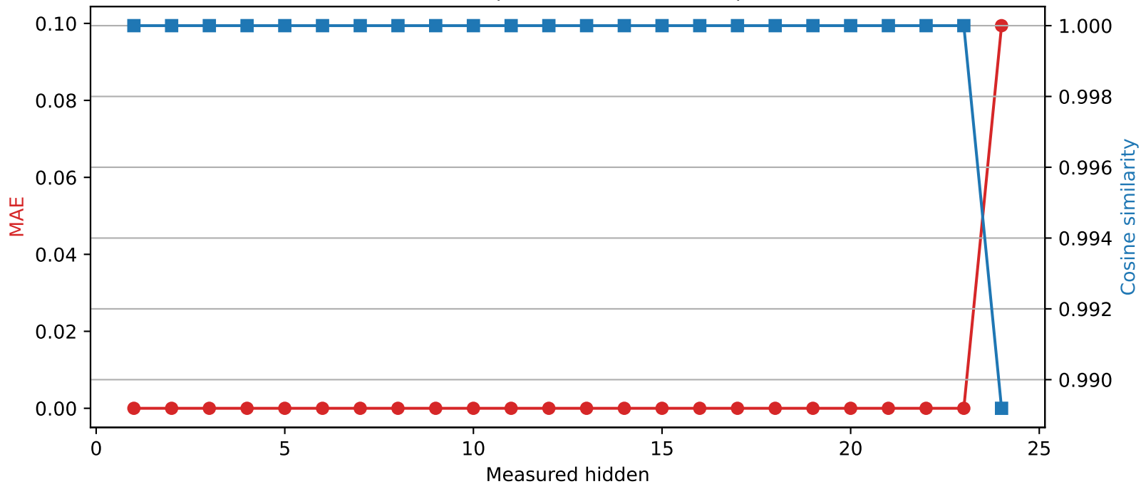
SmolLM2-1.7B-Instruct | Quantized layer 23 | float32 \rightarrow int8
