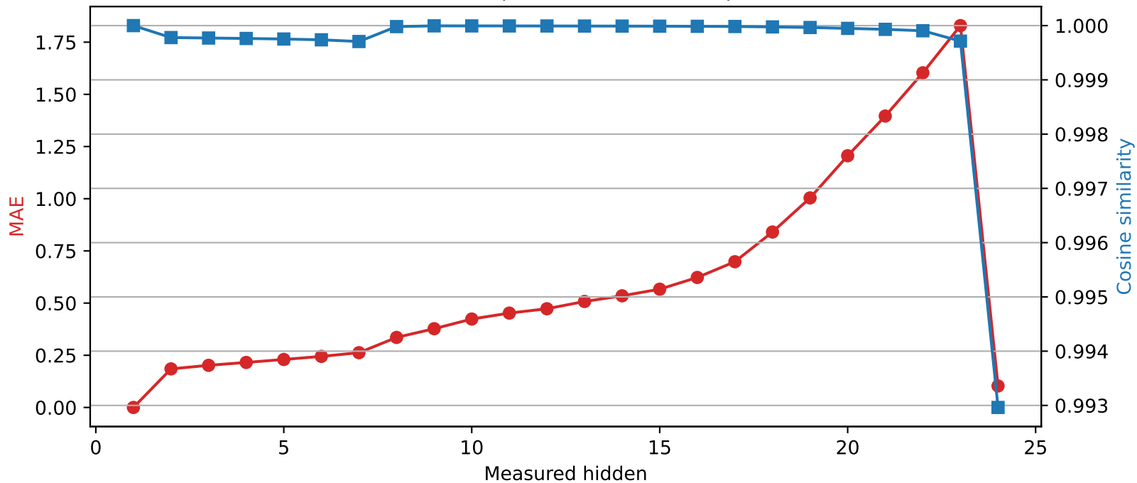
SmolLM2-1.7B-Instruct | Quantized layer 1 | float32 → int8
