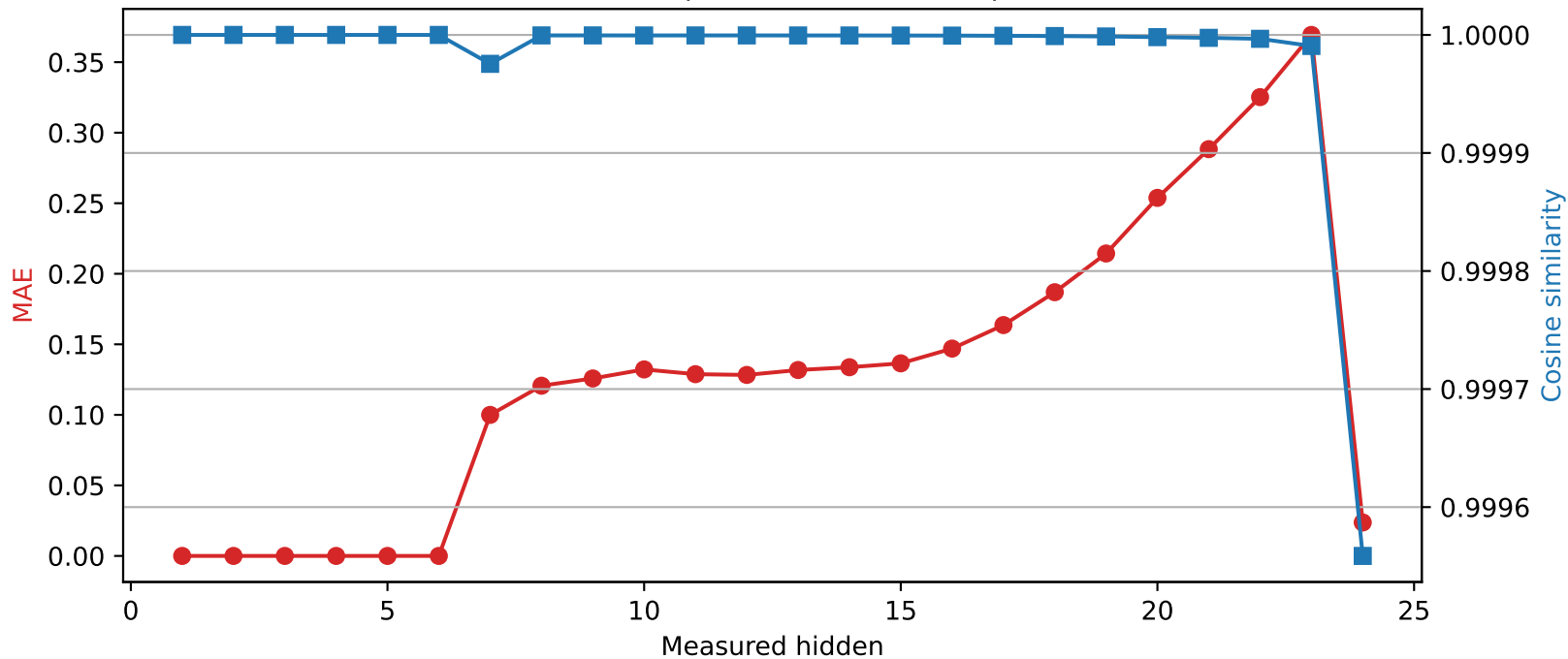
SmolLM2-1.7B-Instruct | Quantized layer 6 | float32 → int8
