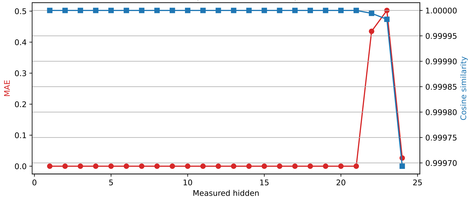
SmolLM2-1.7B-Instruct | Quantized layer 21 | float32 → int8
