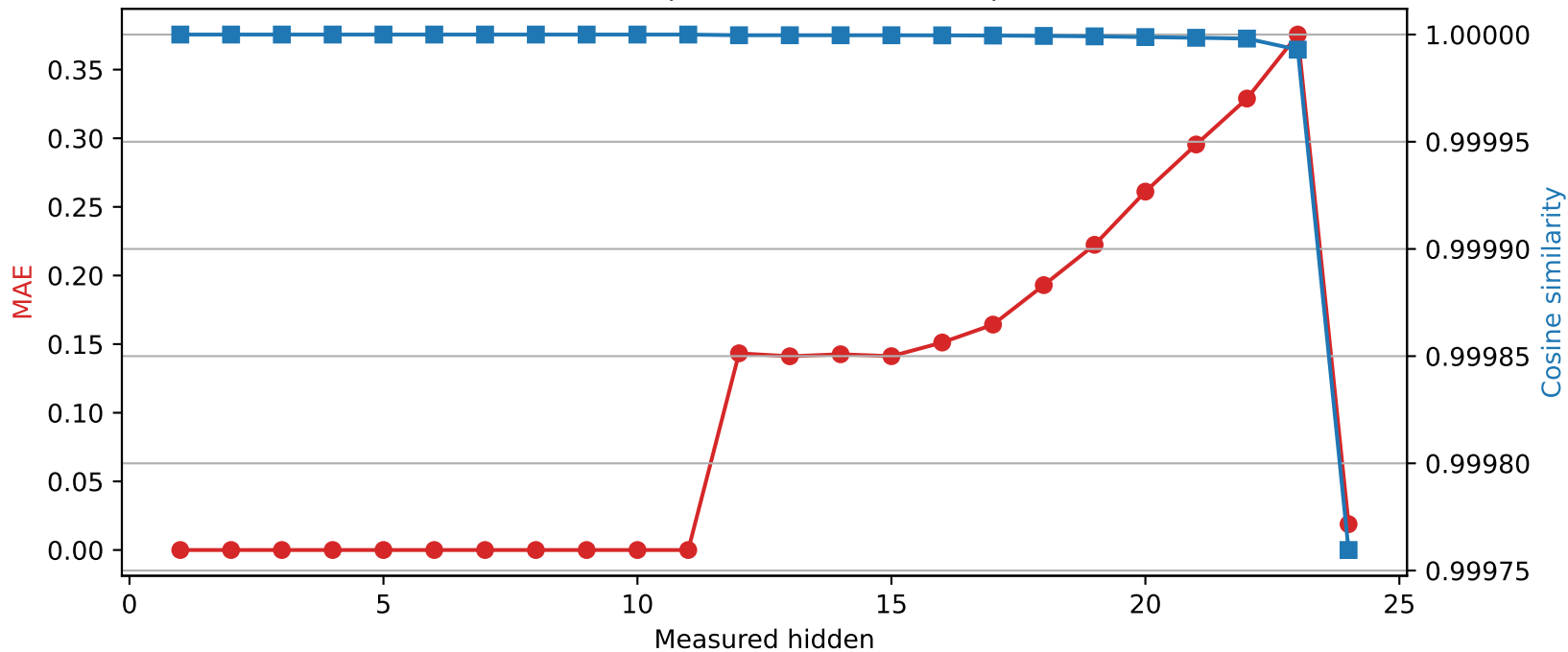
SmolLM2-1.7B-Instruct | Quantized layer 11 | float32 → int8
