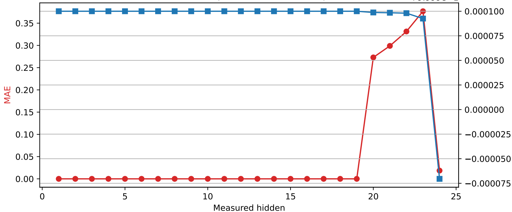
SmolLM2-1.7B-Instruct | Quantized layer 19 | float32 \rightarrow int8
