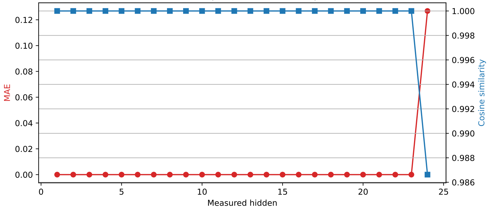
SmolLM2-1.7B-Instruct | Quantized layer 23 | float32 → int8
