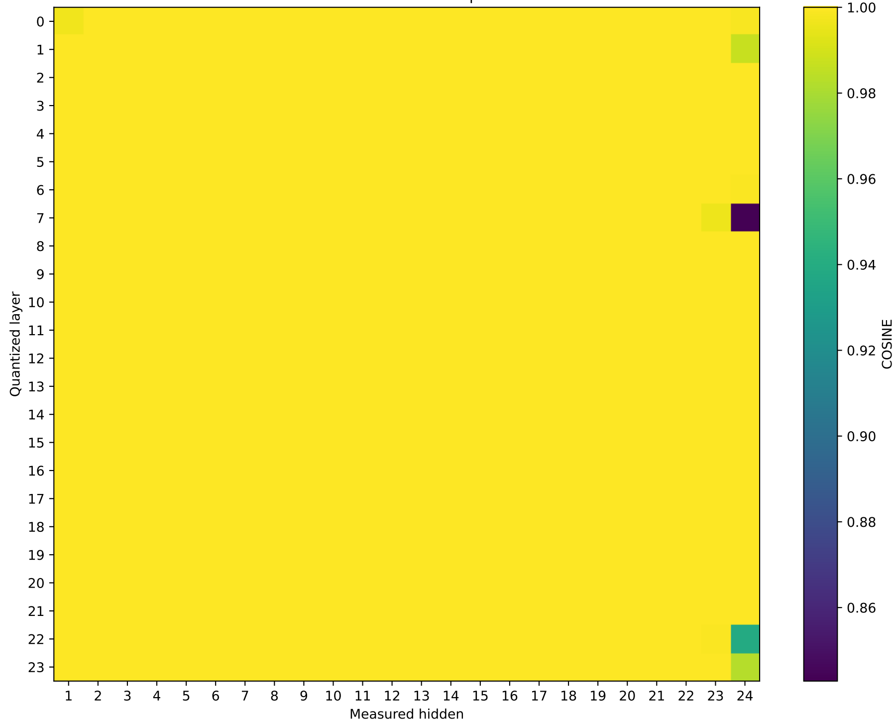
Model: SmolLM2-1.7B-Instruct | float64 → int8
