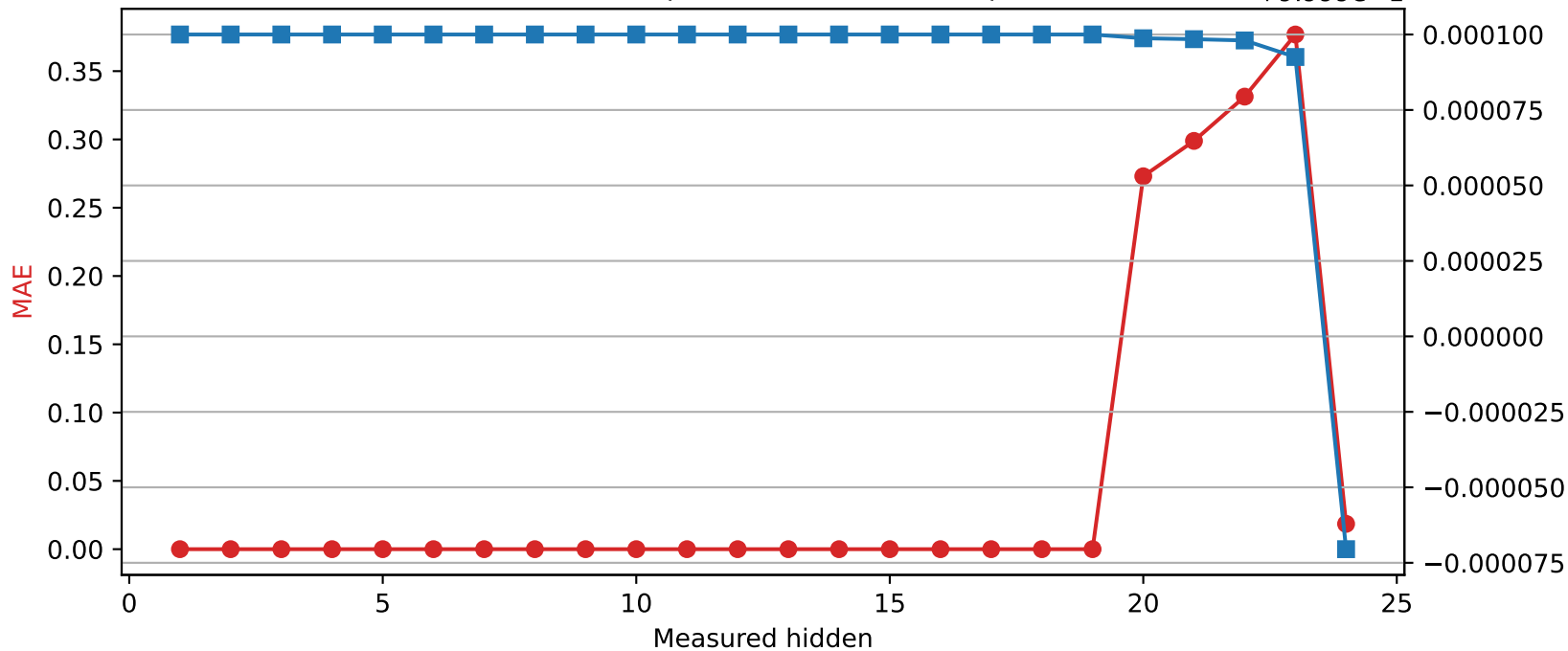
SmolLM2-1.7B-Instruct | Quantized layer 19 | float64 \rightarrow int8
