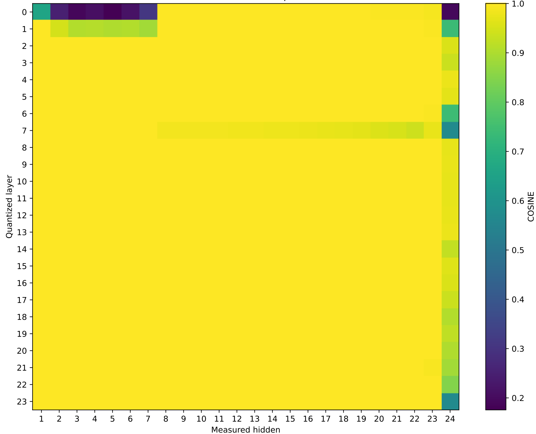
Model: SmolLM2-1.7B-Instruct | float16 → int4
