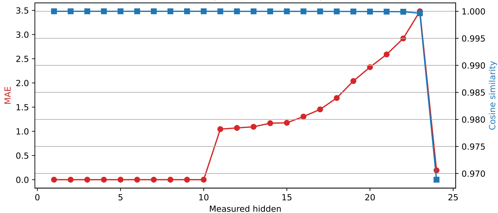
SmolLM2-1.7B-Instruct | Quantized layer 10 | float16 \rightarrow int4
