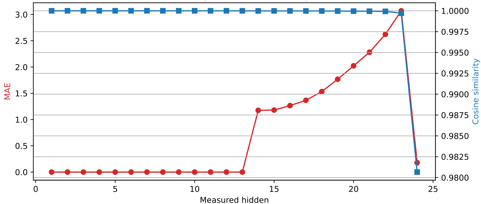
SmolLM2-1.7B-Instruct | Quantized layer 13 | float16 → int4
