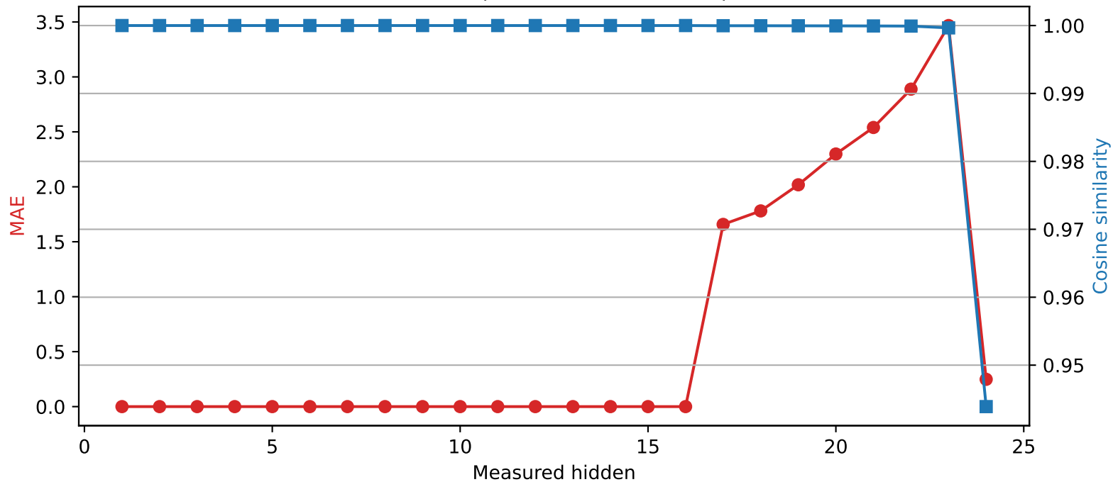
SmolLM2-1.7B-Instruct | Quantized layer 16 | float16 \rightarrow int4
