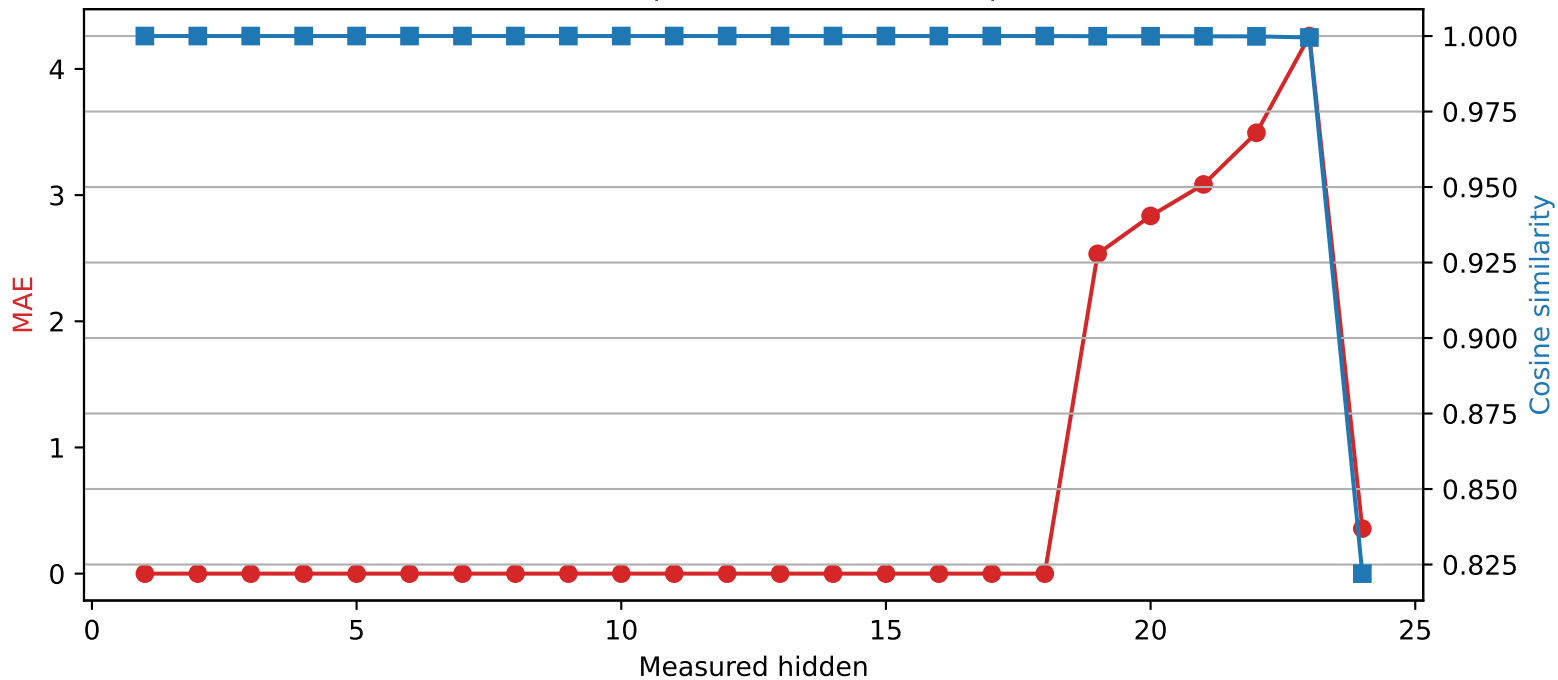
SmolLM2-1.7B-Instruct | Quantized layer 18 | float16 \rightarrow int4
