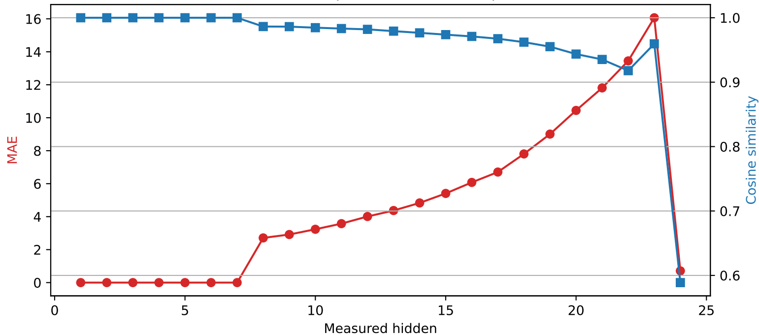
SmolLM2-1.7B-Instruct | Quantized layer 7 | float16 → int4
