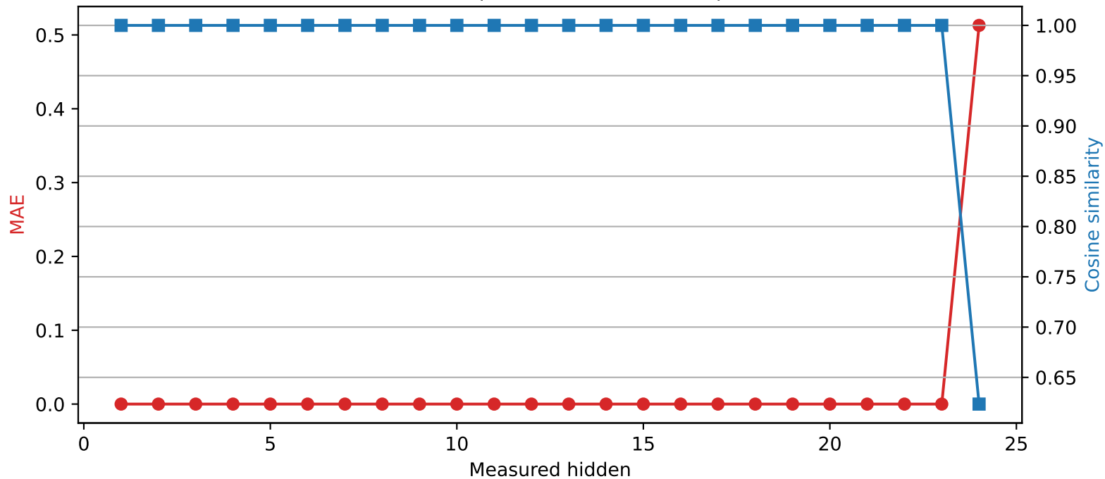
SmolLM2-1.7B-Instruct | Quantized layer 23 | float16 \rightarrow int4
