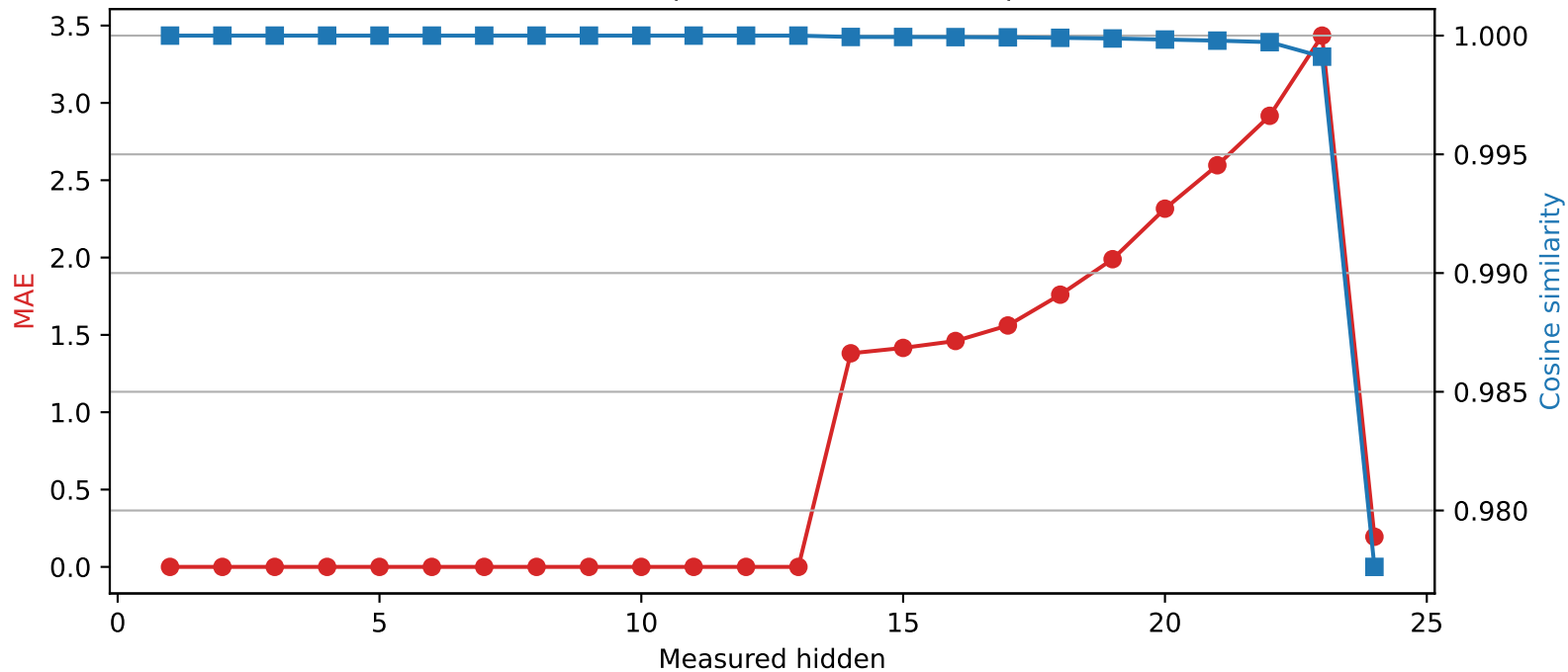
SmolLM2-1.7B-Instruct | Quantized layer 13 | float16 \rightarrow int4
