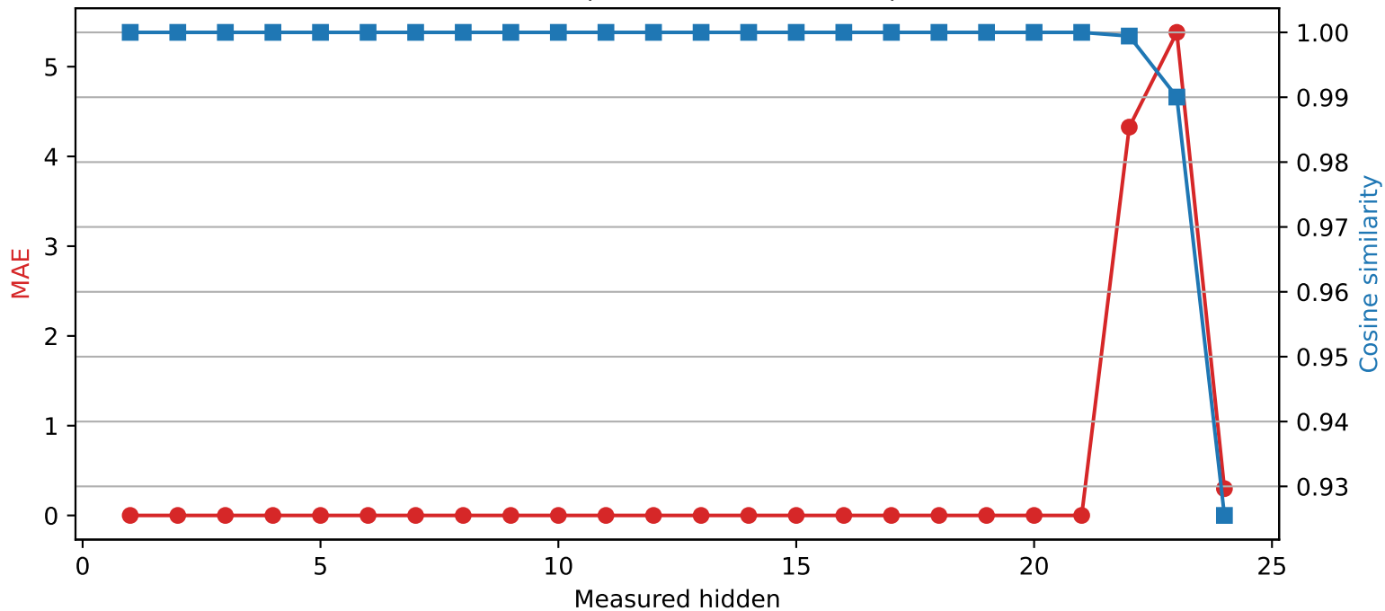
SmolLM2-1.7B-Instruct | Quantized layer 21 | float16 → int4
