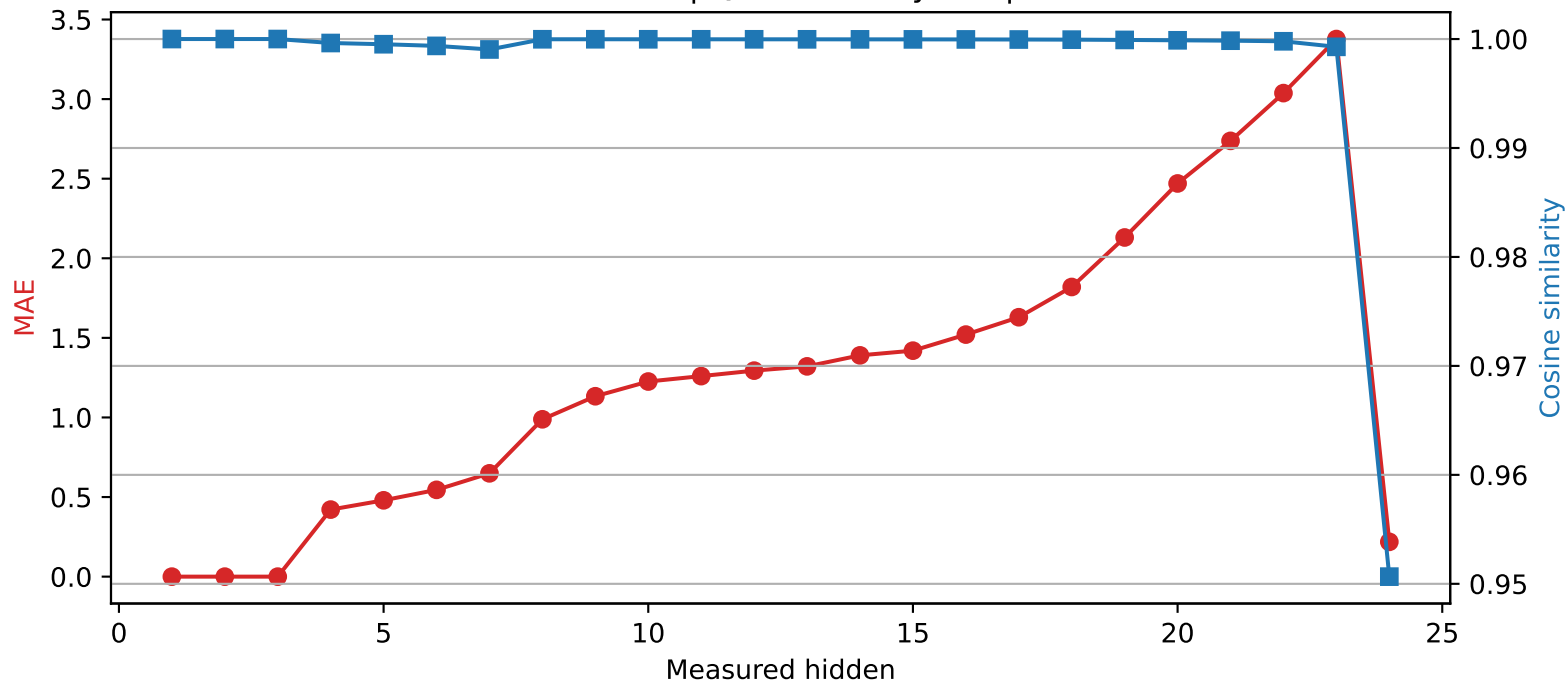
SmolLM2-1.7B-Instruct | Quantized layer 3 | float16 \rightarrow int4
