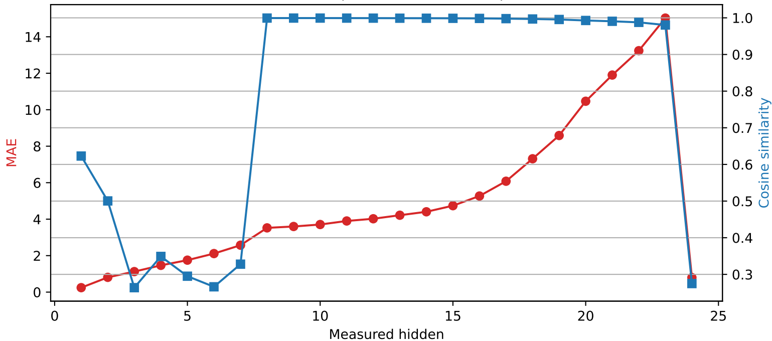
SmolLM2-1.7B-Instruct | Quantized layer 0 | float32 → int4
