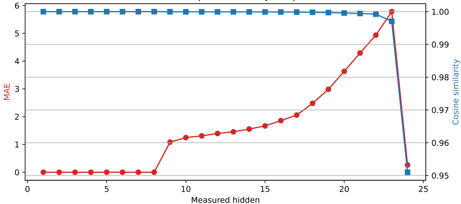
SmolLM2-1.7B-Instruct | Quantized layer 8 | float32 → int4
