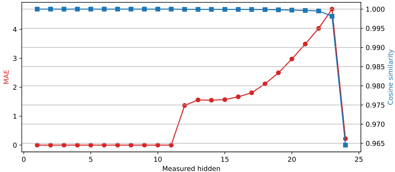
SmolLM2-1.7B-Instruct | Quantized layer 11 | float32 → int4
