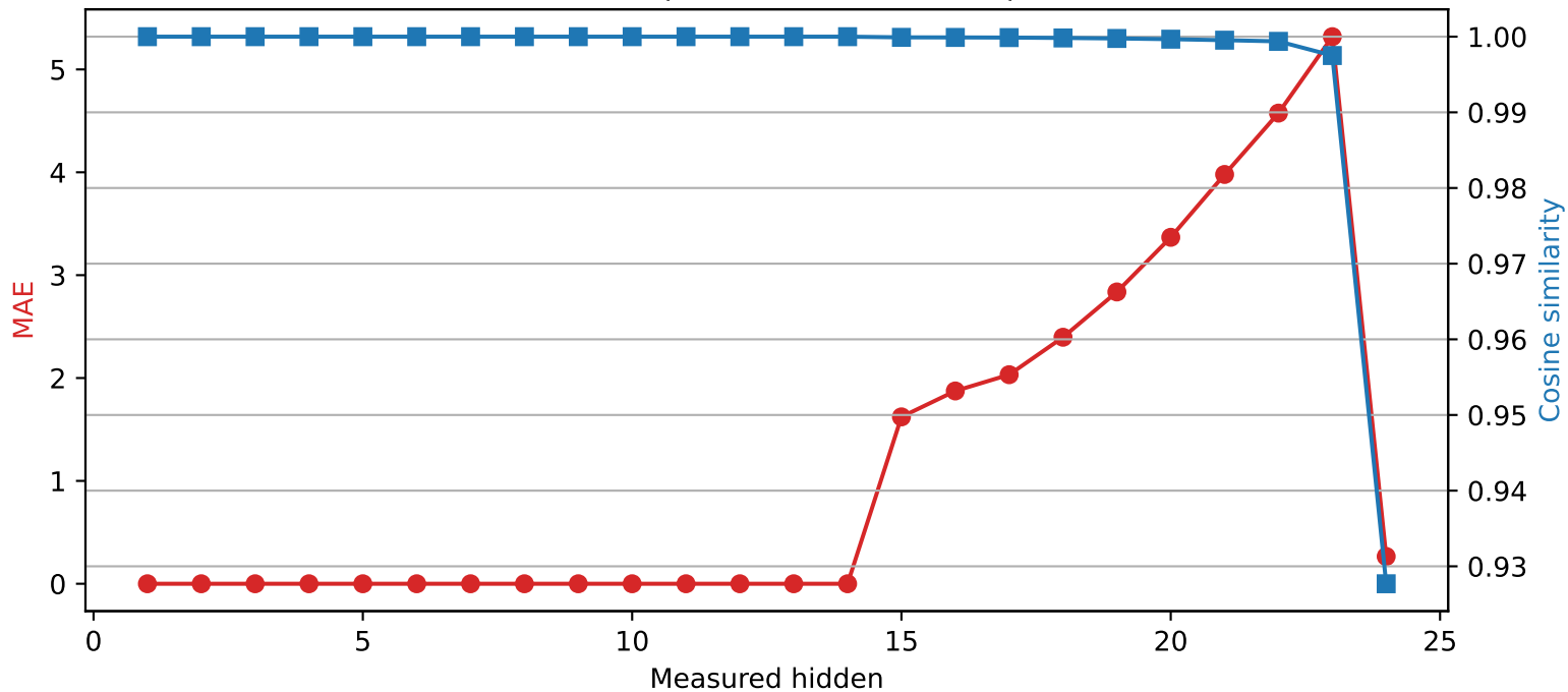
SmolLM2-1.7B-Instruct | Quantized layer 14 | float32 → int4
