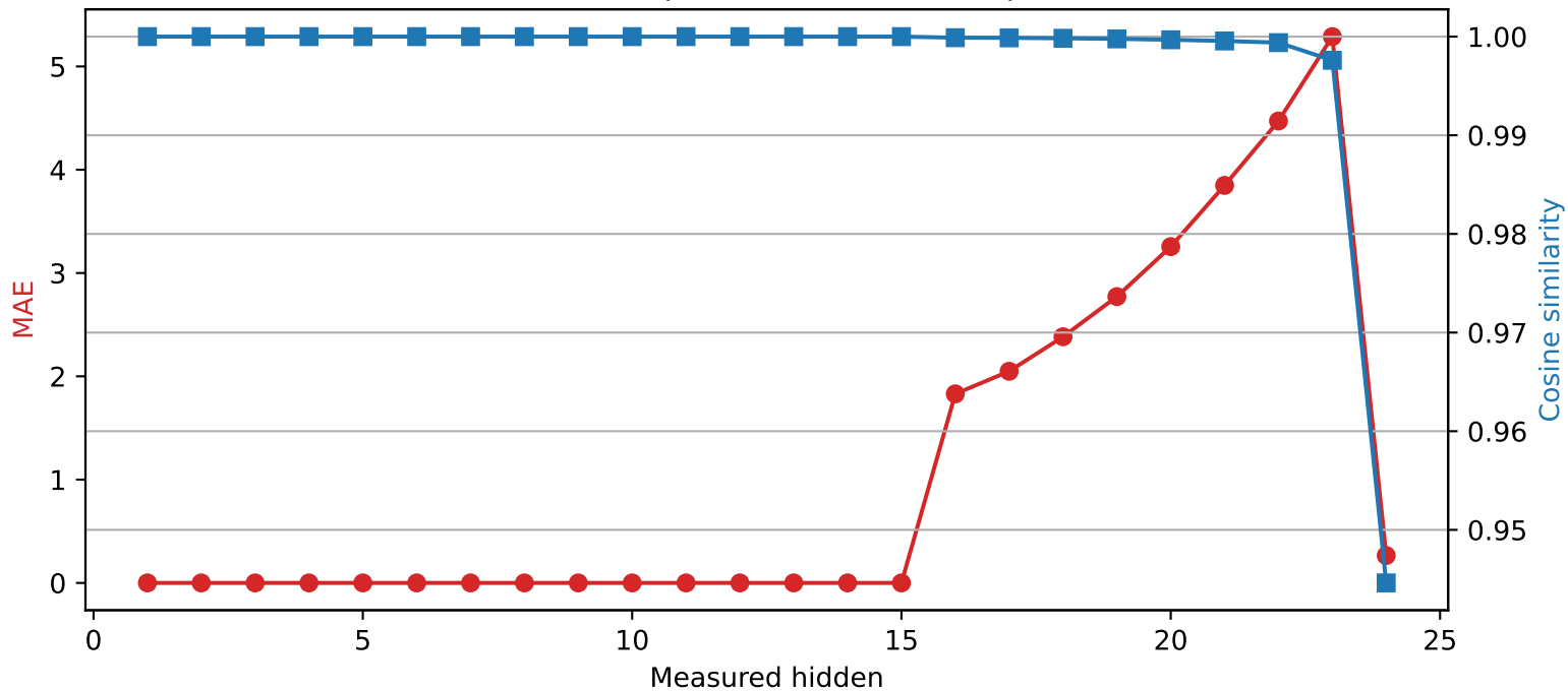
SmolLM2-1.7B-Instruct | Quantized layer 15 | float32 \rightarrow int4
