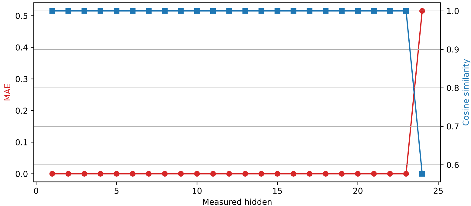
SmolLM2-1.7B-Instruct | Quantized layer 23 | float32 \rightarrow int4
