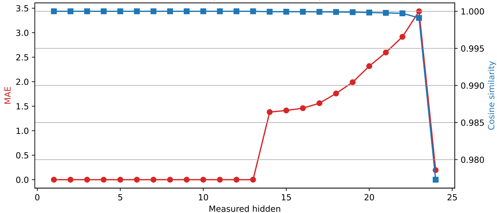
SmolLM2-1.7B-Instruct | Quantized layer 13 | float32 → int4
