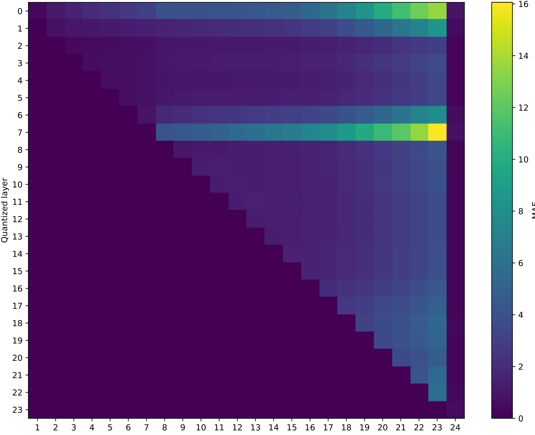
Model: SmolLM2-1.7B-Instruct | float64 → int4
