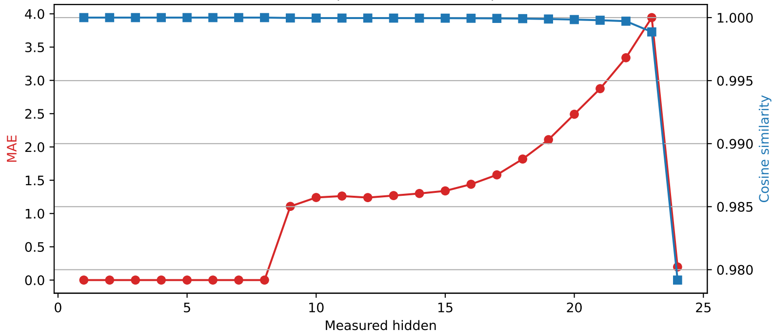
SmolLM2-1.7B-Instruct | Quantized layer 8 | float64 → int4
