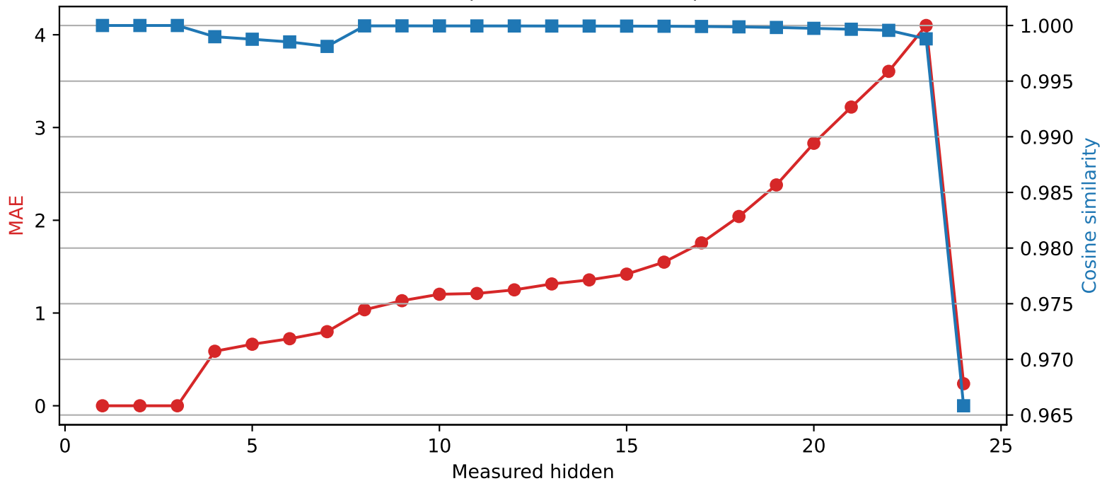
SmolLM2-1.7B-Instruct | Quantized layer 3 | float64 → int4
