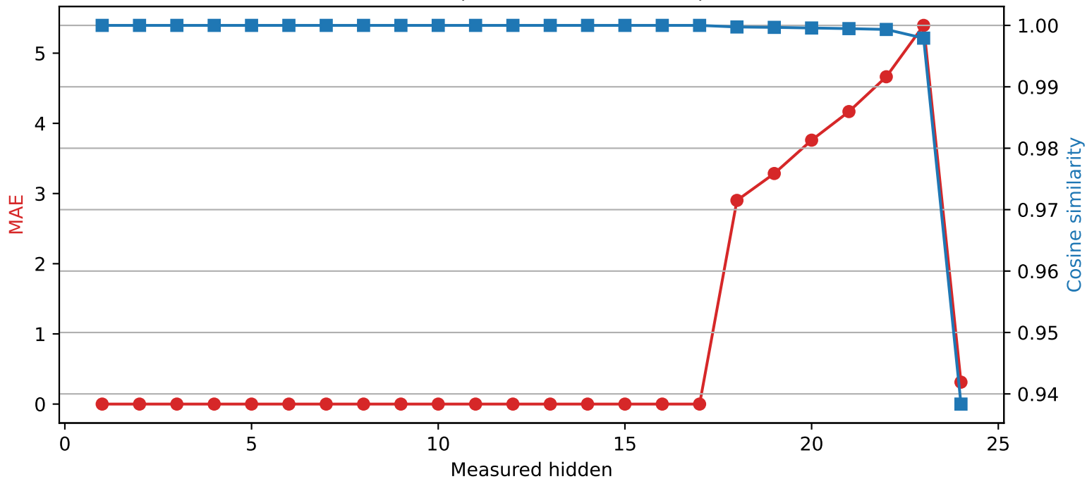
SmolLM2-1.7B-Instruct | Quantized layer 17 | float64 → int4
