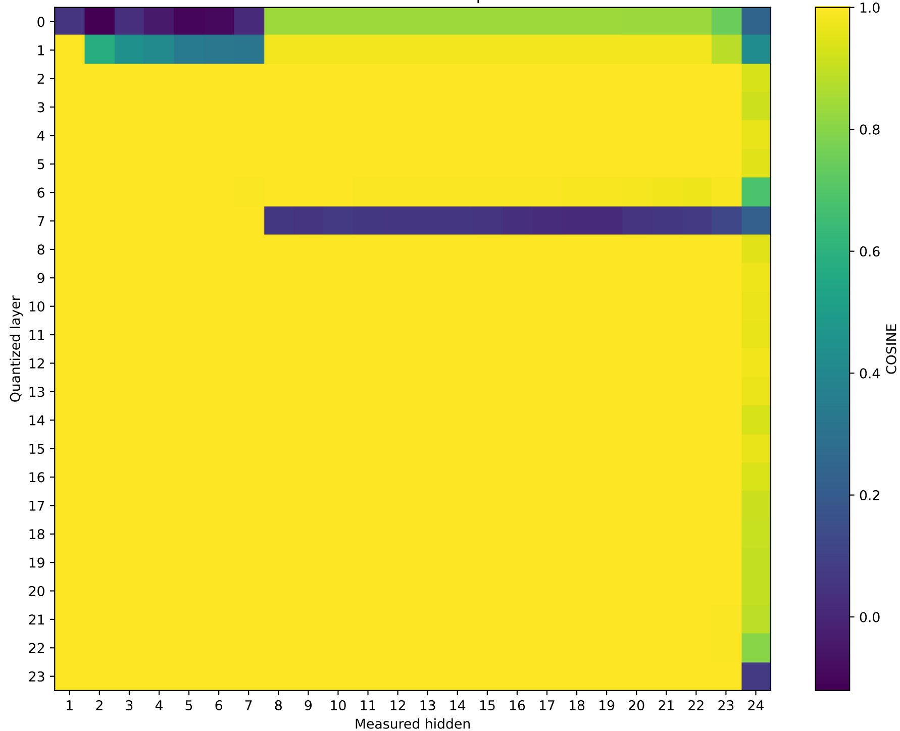
Model: SmolLM2-1.7B-Instruct | float16 \rightarrow int2
