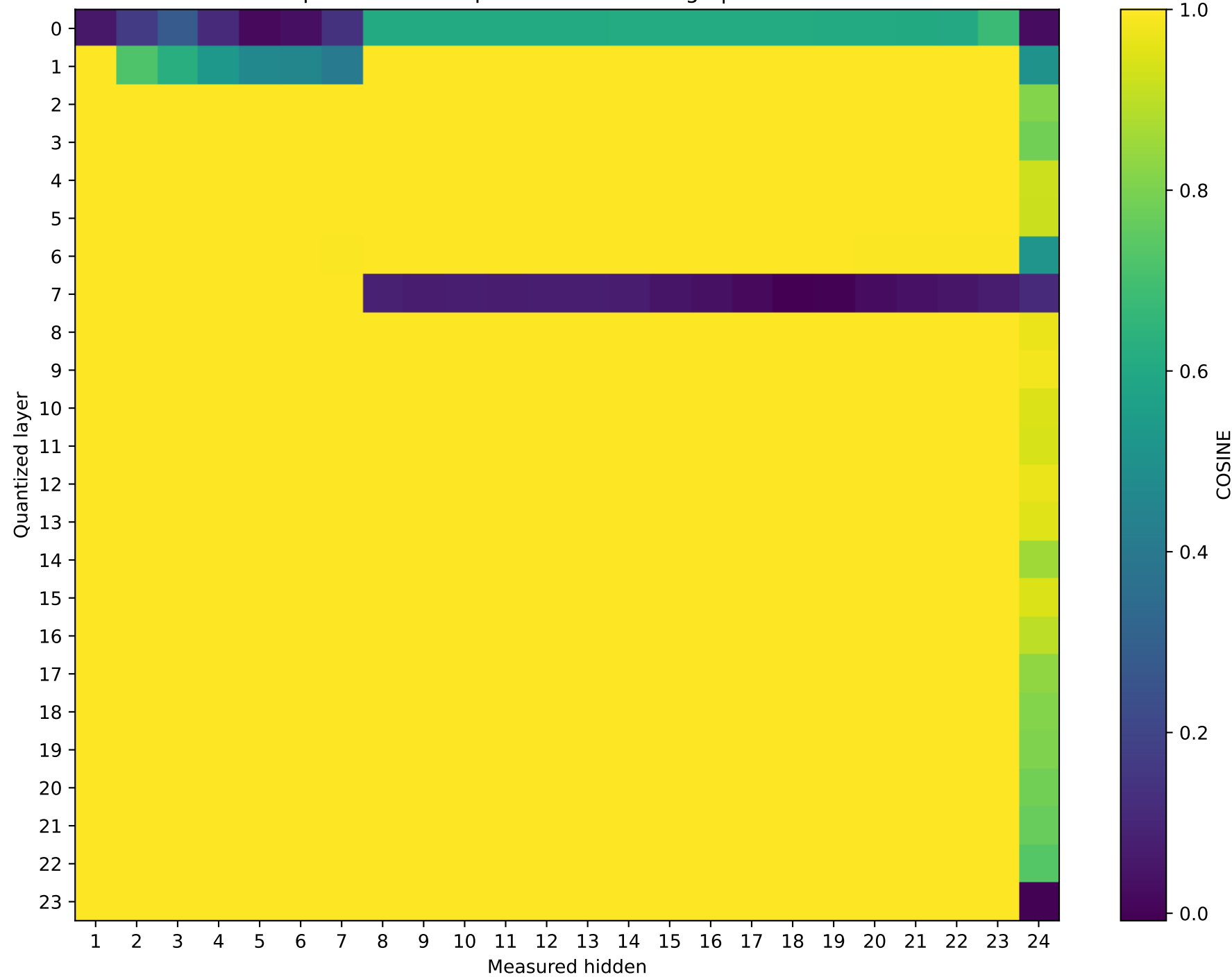
SmolLM2-1.7B-Instruct Prompt 0: cos sim representation damage | float16 → int2
