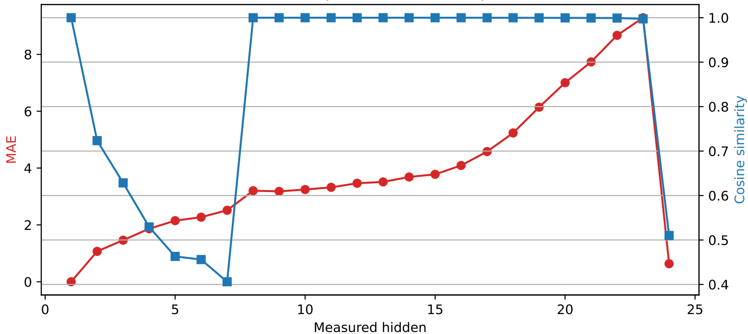
SmolLM2-1.7B-Instruct | Quantized layer 1 | float16 → int2
