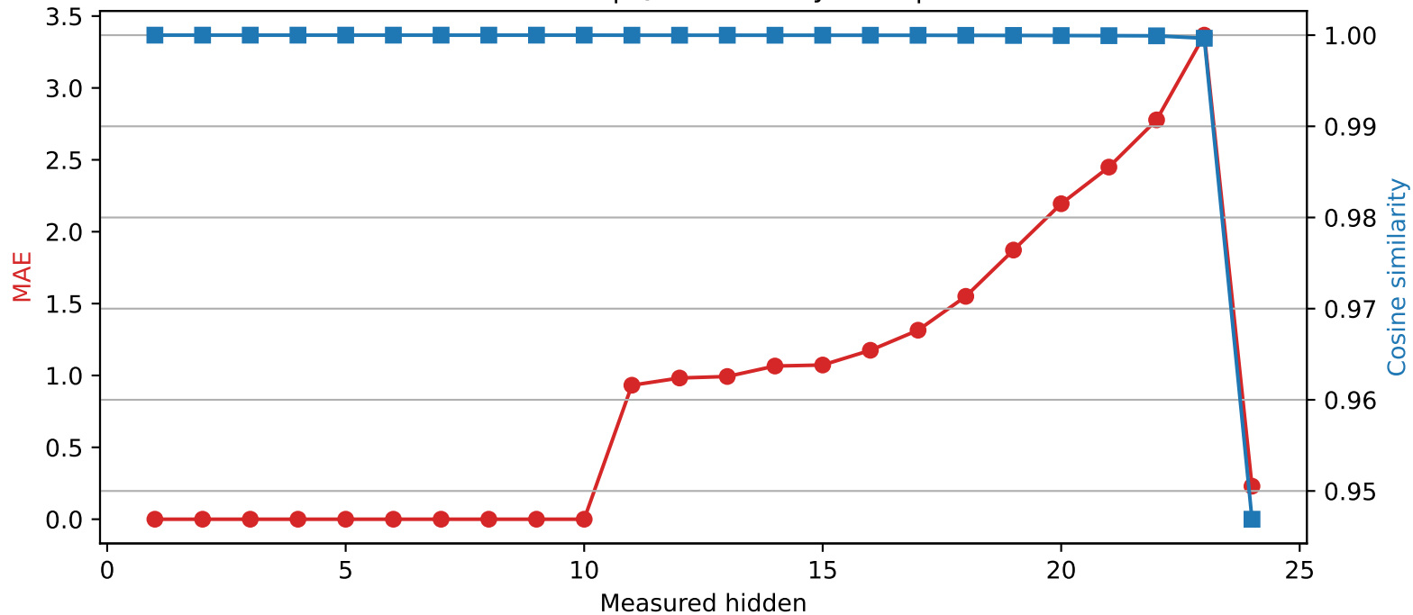
SmolLM2-1.7B-Instruct | Quantized layer 10 | float16 \rightarrow int2
