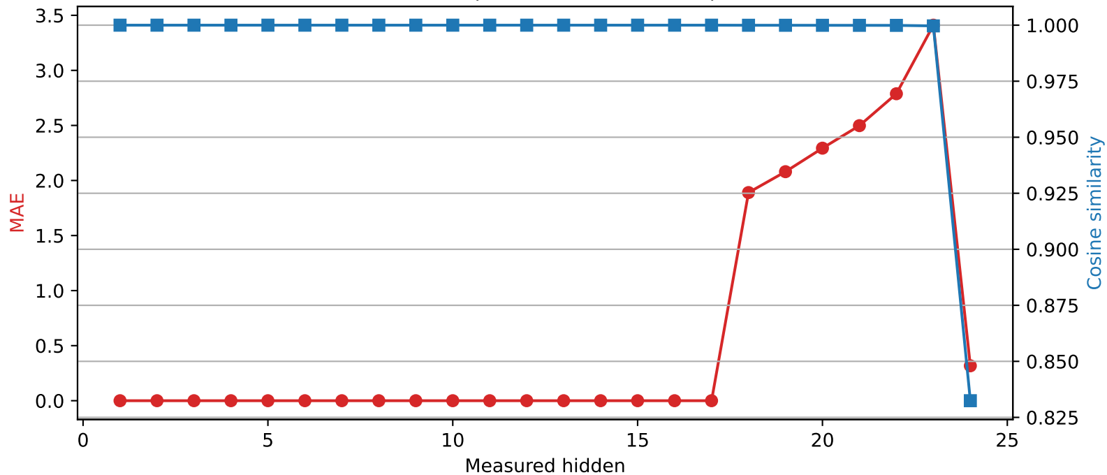
SmolLM2-1.7B-Instruct | Quantized layer 17 | float16 \rightarrow int2
