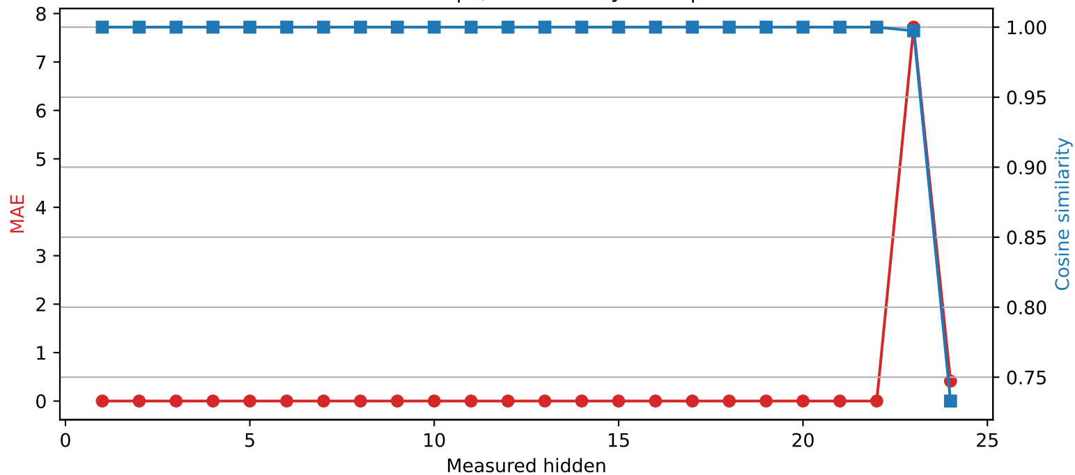
SmolLM2-1.7B-Instruct | Quantized layer 22 | float16 → int2
