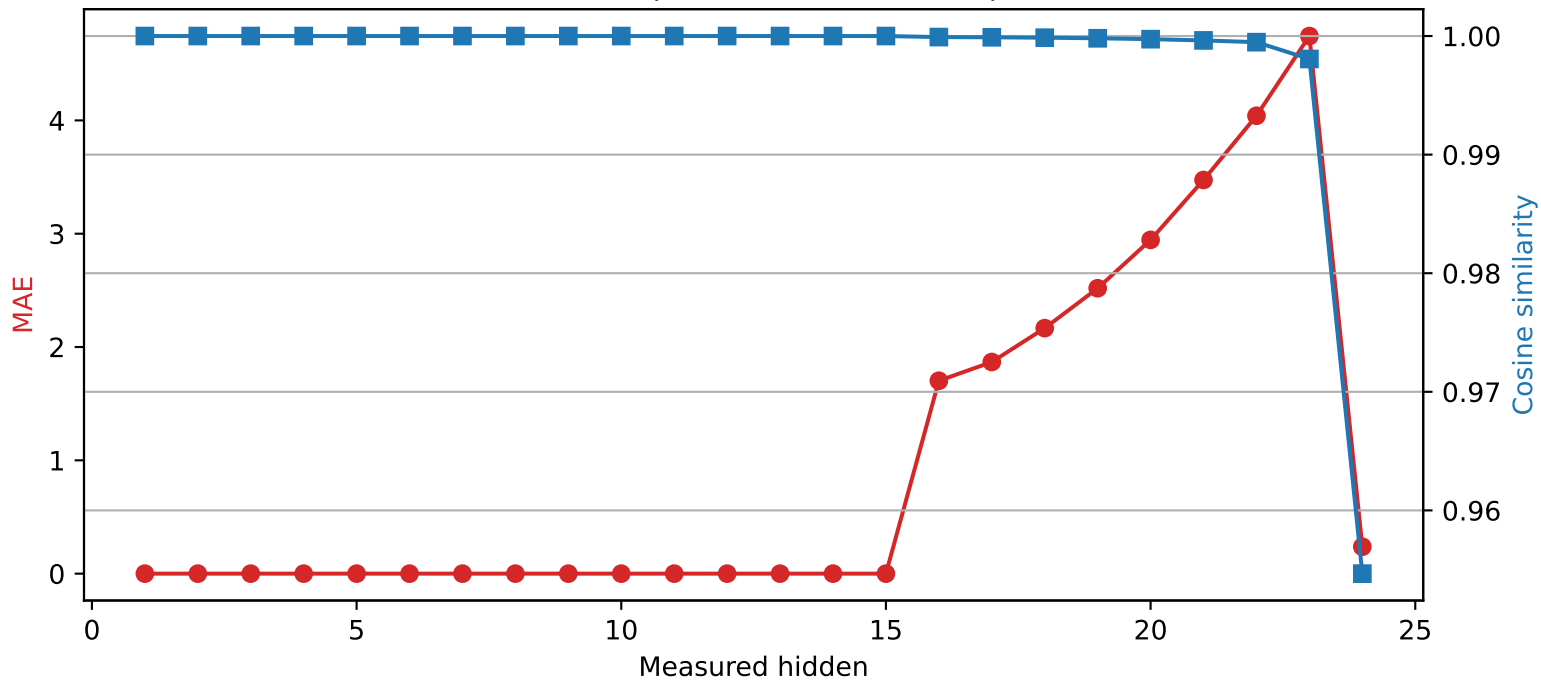
SmolLM2-1.7B-Instruct | Quantized layer 15 | float16 → int2
