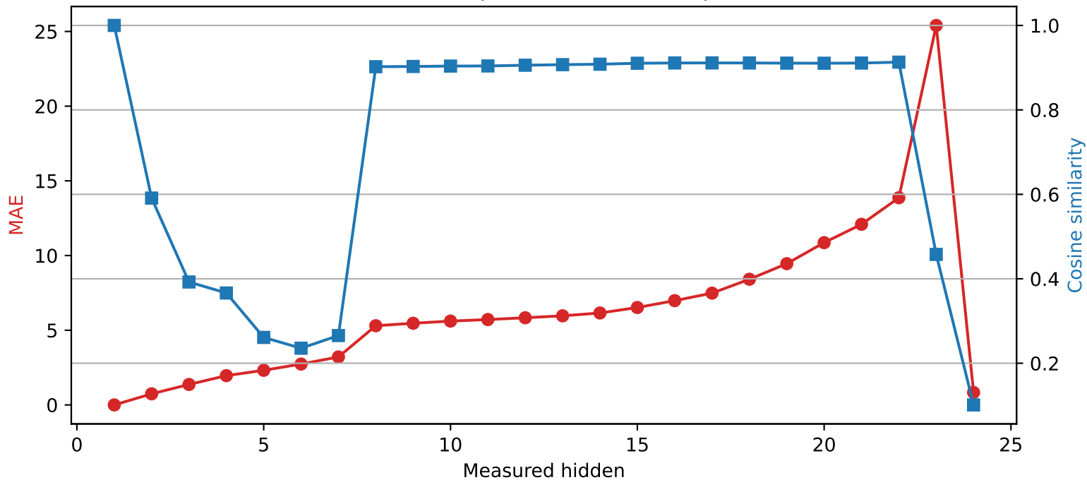
SmolLM2-1.7B-Instruct | Quantized layer 1 | float16 \rightarrow int2
