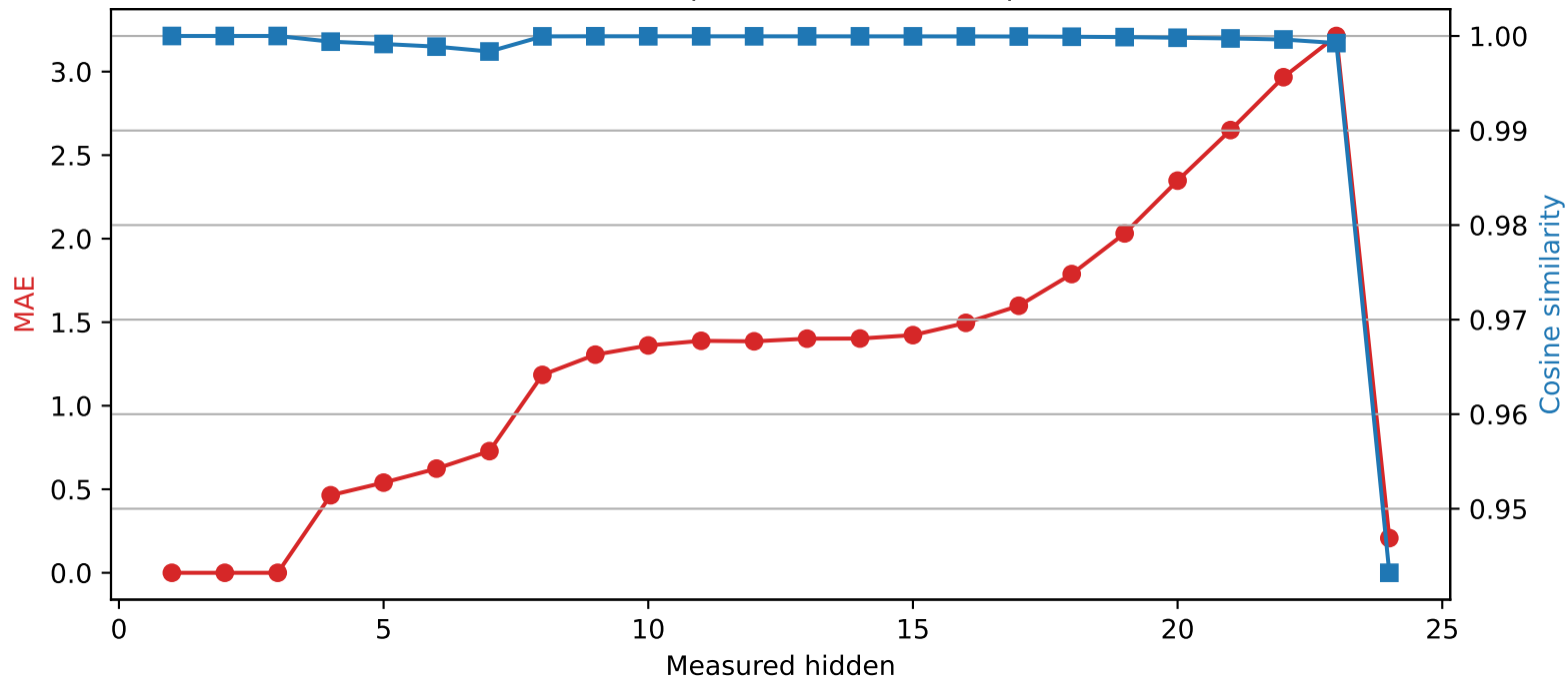
SmolLM2-1.7B-Instruct | Quantized layer 3 | float16 \rightarrow int2
