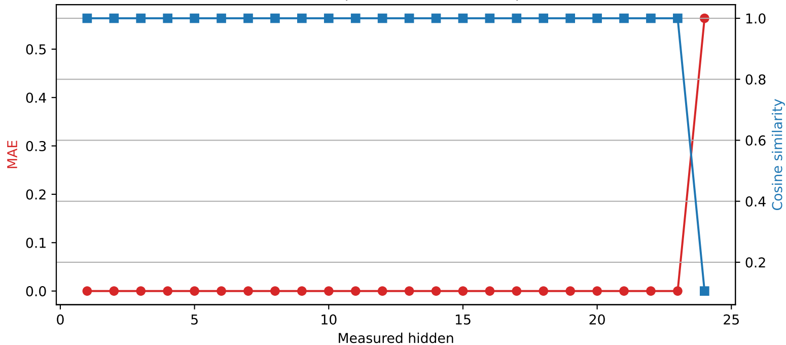
SmolLM2-1.7B-Instruct | Quantized layer 23 | float32 → int2
