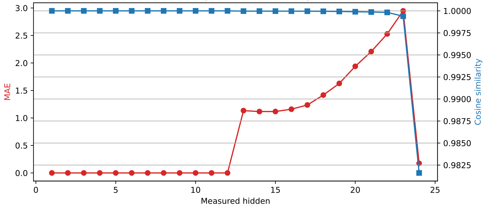
SmolLM2-1.7B-Instruct | Quantized layer 12 | float32 → int2
