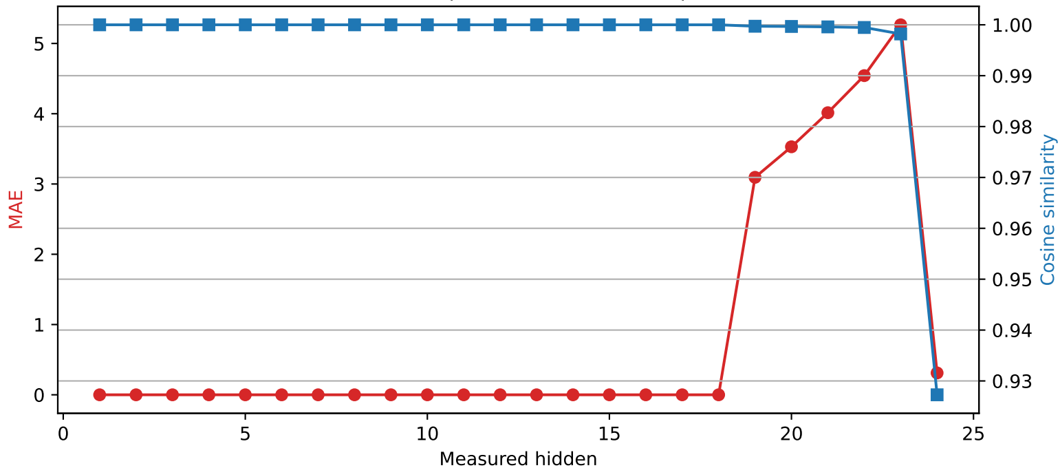
SmolLM2-1.7B-Instruct | Quantized layer 18 | float32 \rightarrow int2
