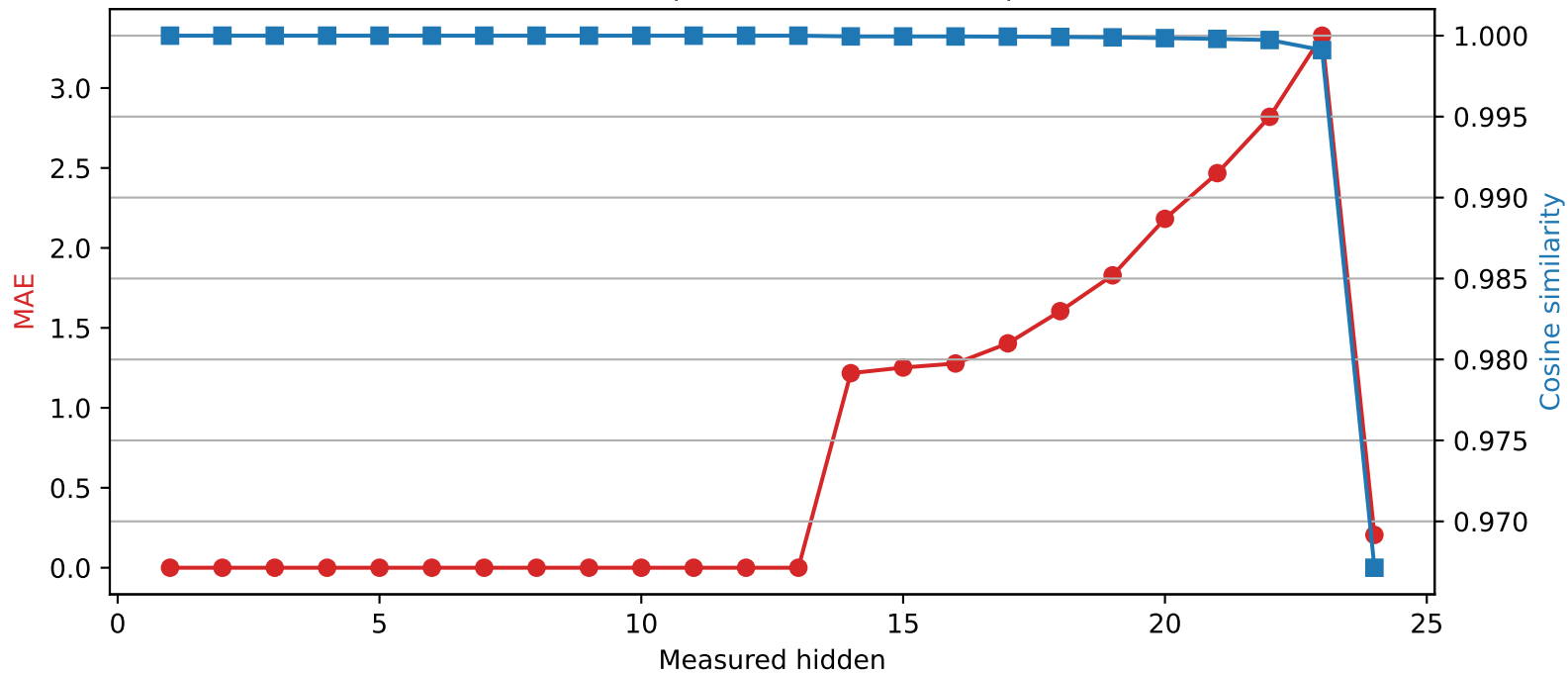
SmolLM2-1.7B-Instruct | Quantized layer 13 | float32 → int2
