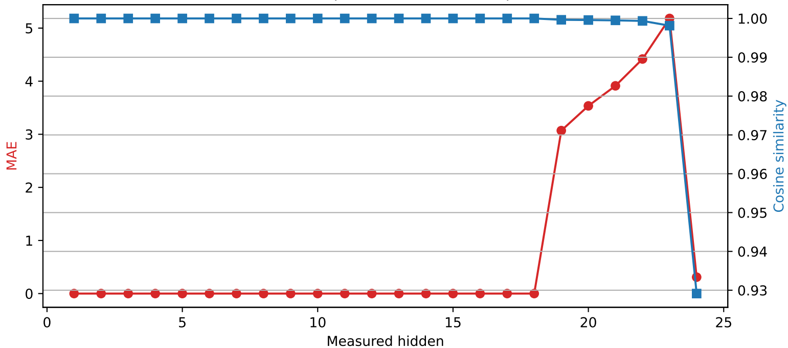
SmolLM2-1.7B-Instruct | Quantized layer 18 | float32 → int2
