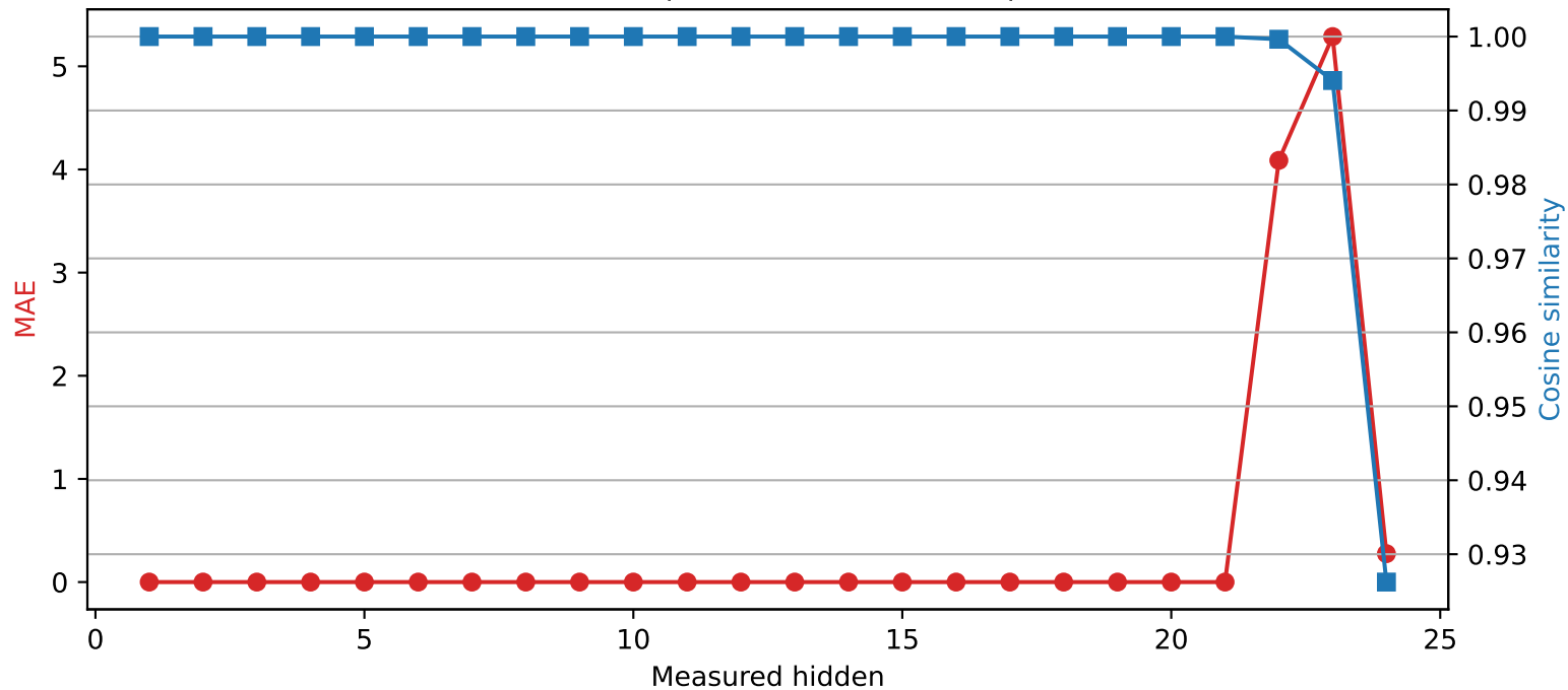
SmolLM2-1.7B-Instruct | Quantized layer 21 | float32 → int2
