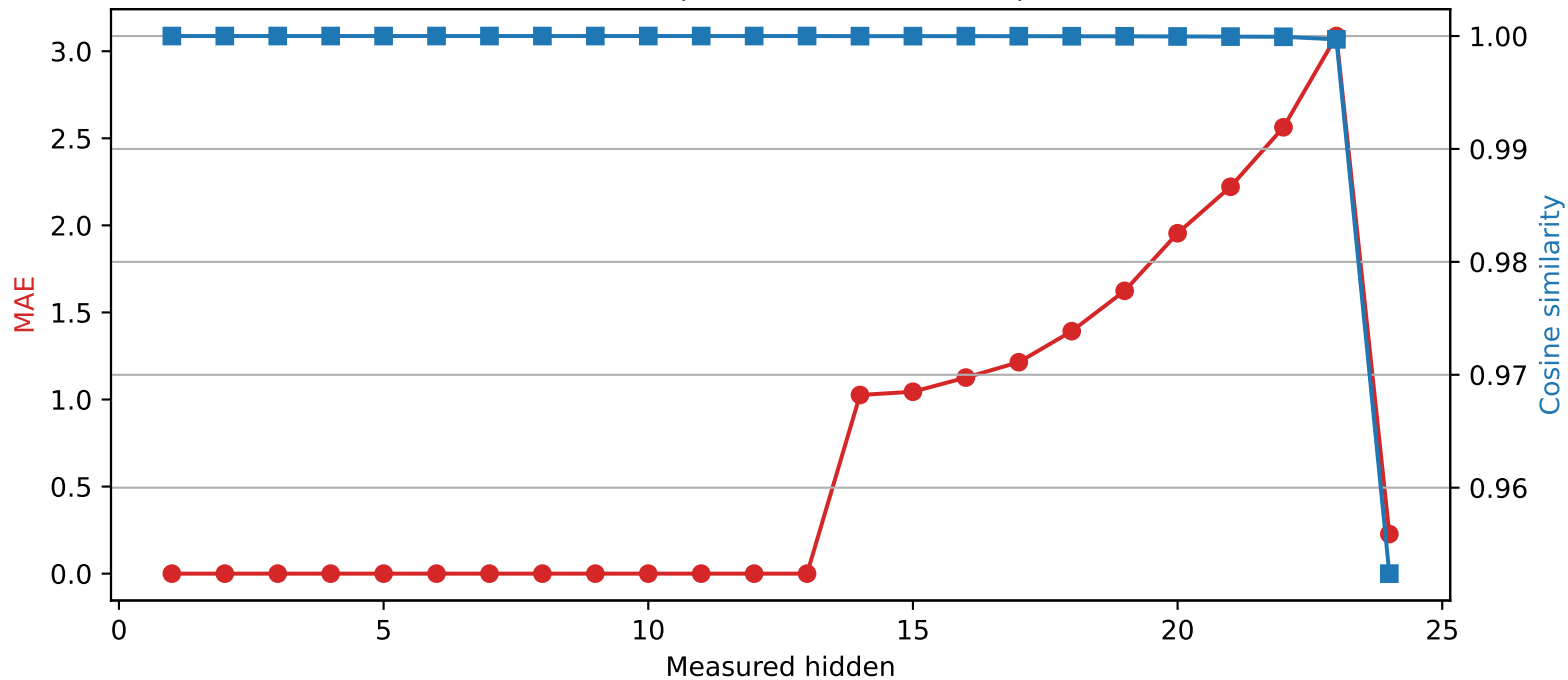
SmolLM2-1.7B-Instruct | Quantized layer 13 | float64 \rightarrow int2
