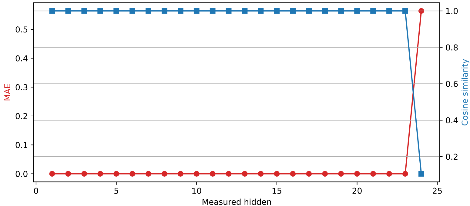
SmolLM2-1.7B-Instruct | Quantized layer 23 | float64 → int2
