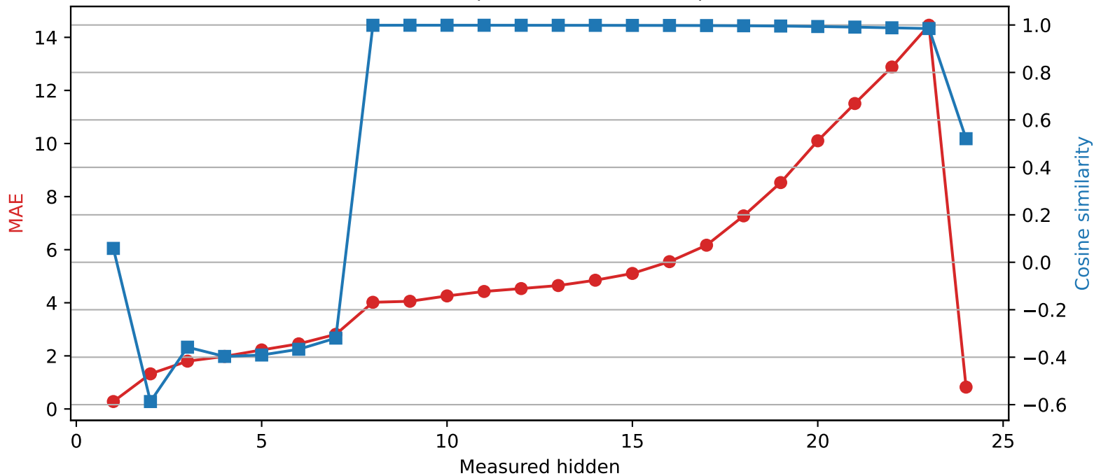
SmolLM2-1.7B-Instruct | Quantized layer 0 | float64 → int2
