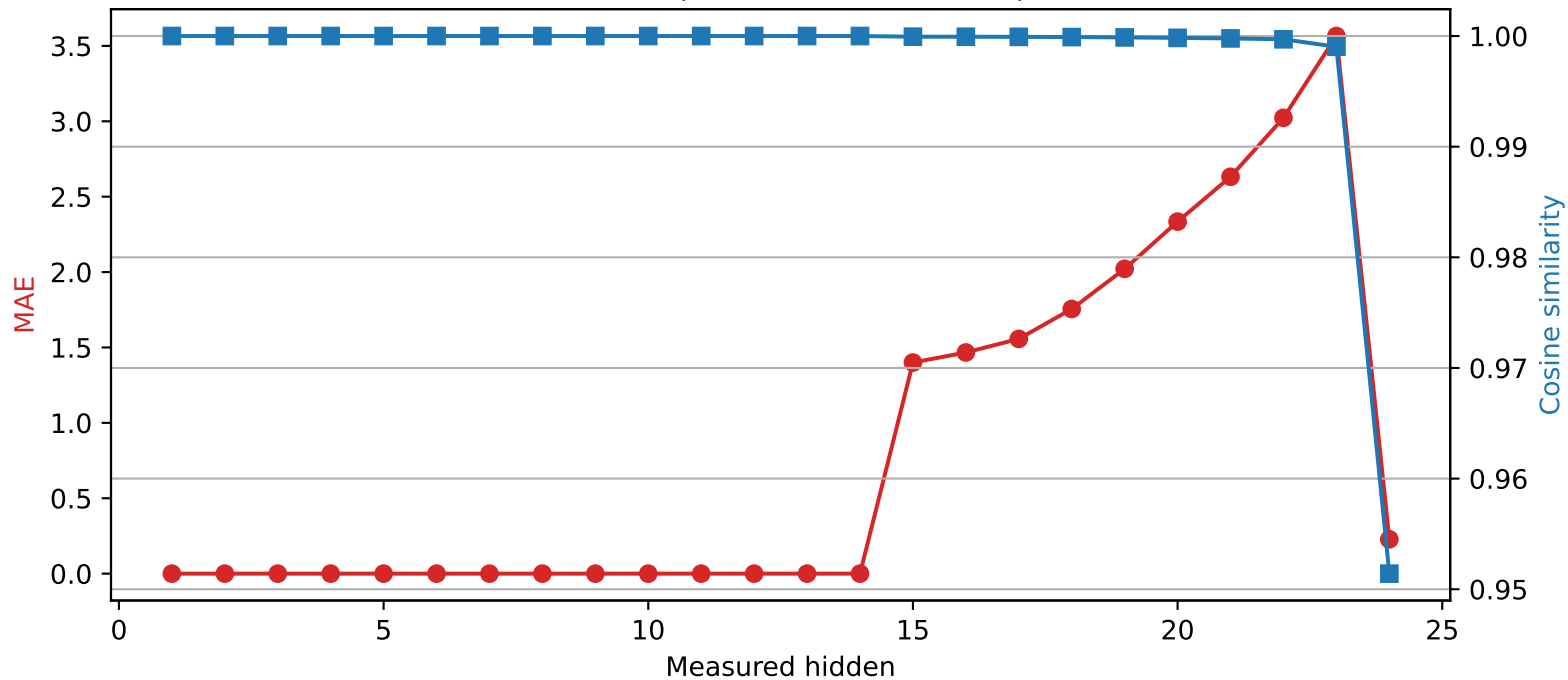
SmolLM2-1.7B-Instruct | Quantized layer 14 | float64 → int2
